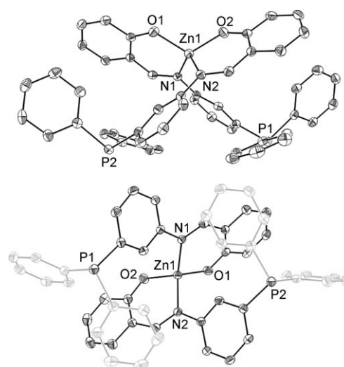
Figure 1. ORTEP plot of the molecular structure of 12 in two different projections. Thermal ellipsoids are set at the 50% probability level; hydrogen atoms are omitted for clarity. Selected interatomic separations [Å] and bond angles [°]: P1–P2 7.7; N1–Zn1–O1 97.45(8), O1–Zn1–O2 117.20(8), N1–Zn1–N2 118.82(8), N2–Zn1–O2 98.05(8).
